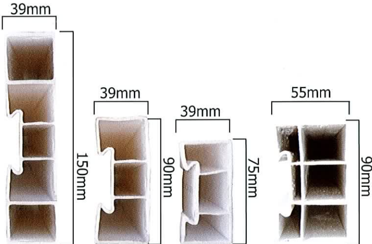
Flexible Boards
